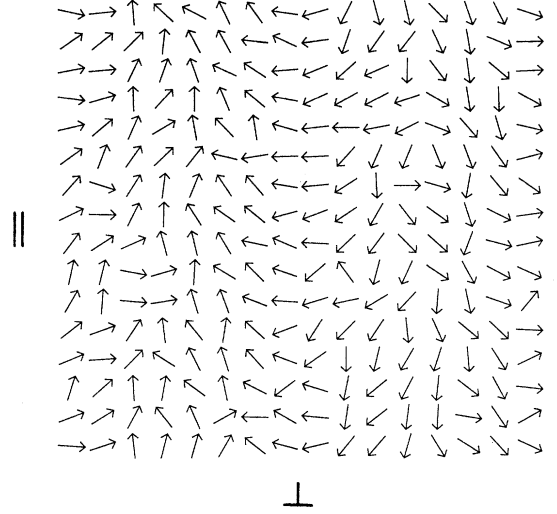
FIG. 1. A typical ordered configuration with long-range order. The \perp and \parallel directions correspond to the directions of the \perp and \parallel bonds, respectively. The configuration shows a spin wave in the perpendicular direction.
