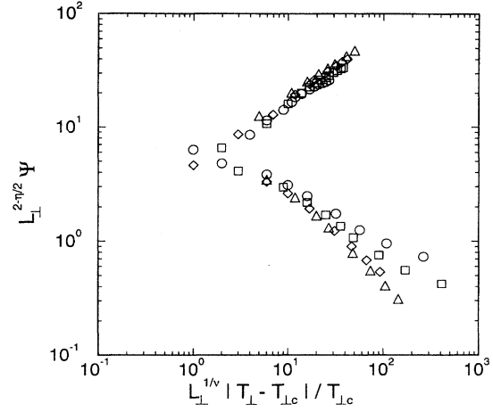
FIG. 4. Finite-size scaling of Monte Carlo results for the order parameter \langle \Psi \rangle , using \beta_{\perp c} = 0.68 , \nu = 0.65 , and \eta = 0.02 . The size and shape, L_{\perp} \times L_{\parallel} , of the systems is the same as in Fig. 2.
