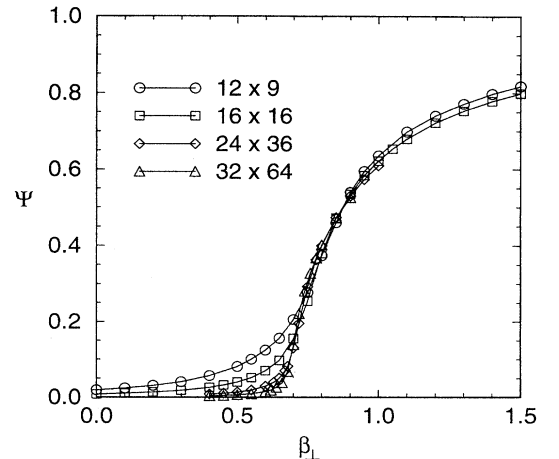
FIG. 2. Monte Carlo results for the order parameter \langle \Psi \rangle , showing a transition to long-range order at \beta_{\perp,c} \approx 0.68 . The size and shape ( L_{\perp} \times L_{\parallel} ) of the systems is indicated in the legend. Error bars are much smaller than the symbol size.
